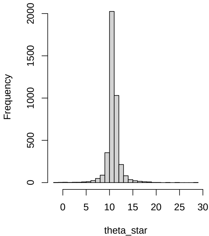
Irregular AR( 1) predictive draws for \theta_{\text{star}}
